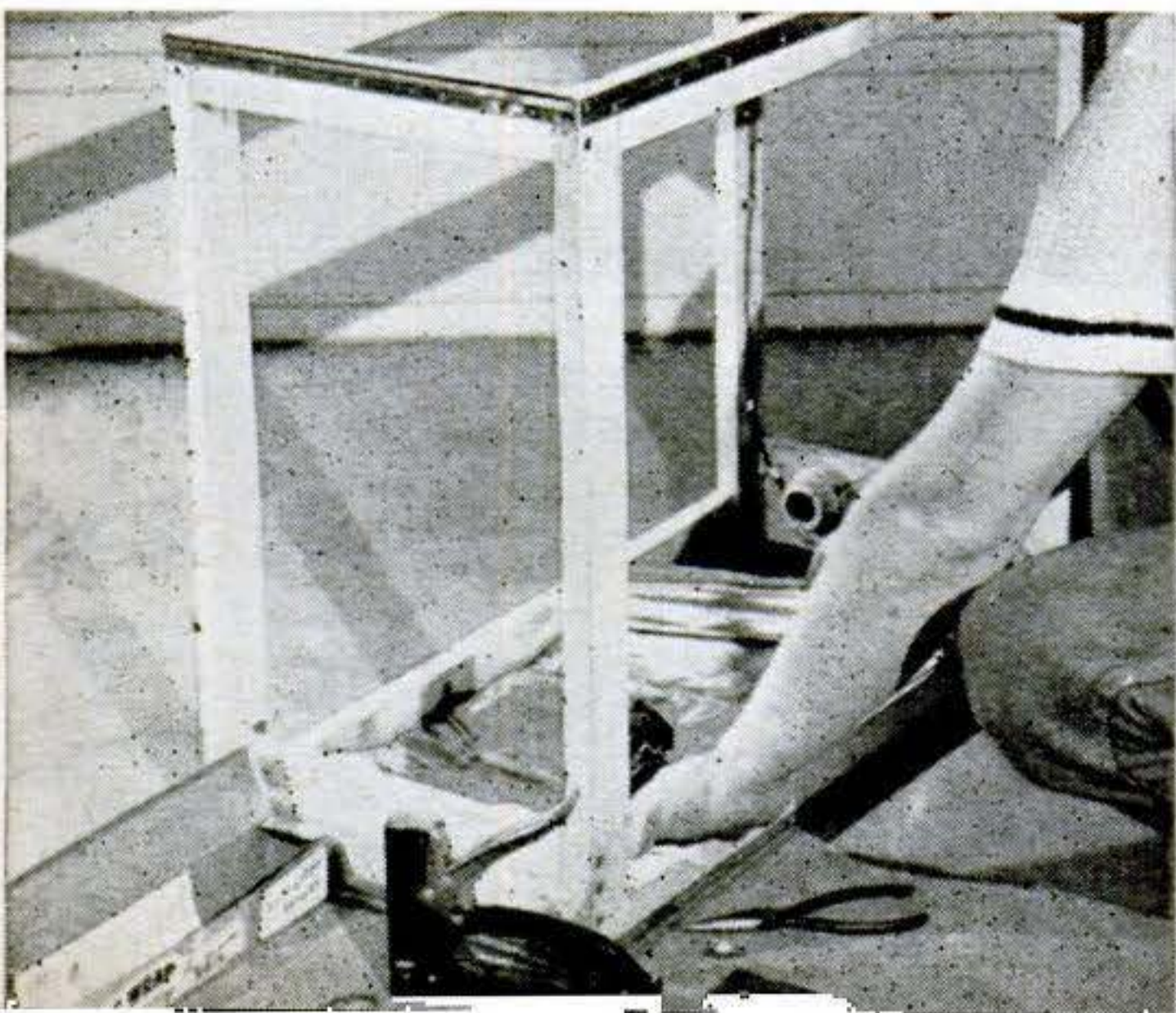
LINOLEUM CAP MOLDING is nailed all around top and bottom of frame to receive panels. Bottom is lined with aluminum foil.
